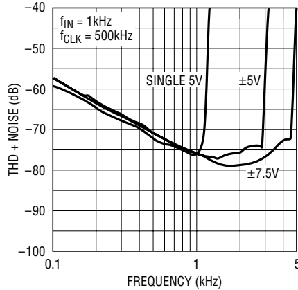
LTC1164-5 • G16
