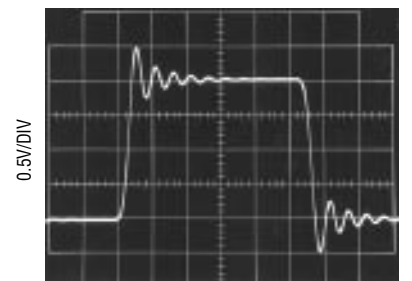
Transient Response
