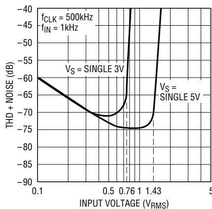
Dynamic Range THD + Noise vs Input Voltage
