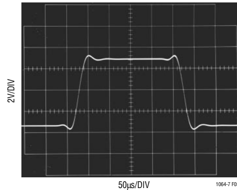
V_S = \pm 7.5V , f_{IN} = 2kHz \pm 3V f_{CLK} = 1MHz , RATIO = 50:1
