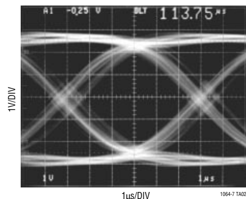
Eye Diagram
