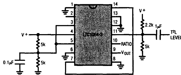
Figure 4. Level Shifting the Input T²L Clock for Single Supply Operation ≥ 6V.
