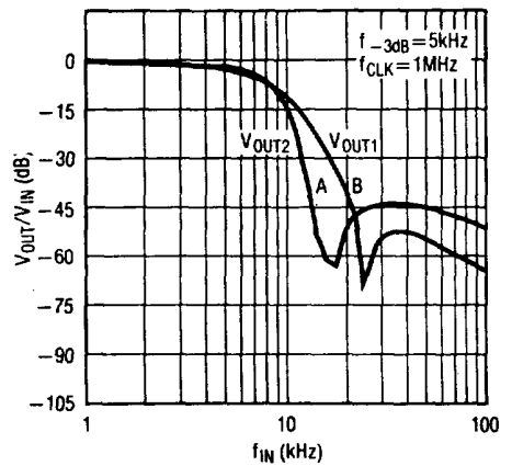
Amplitude Response
