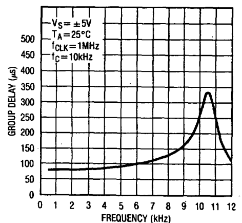
Graph 3. Group Delay
