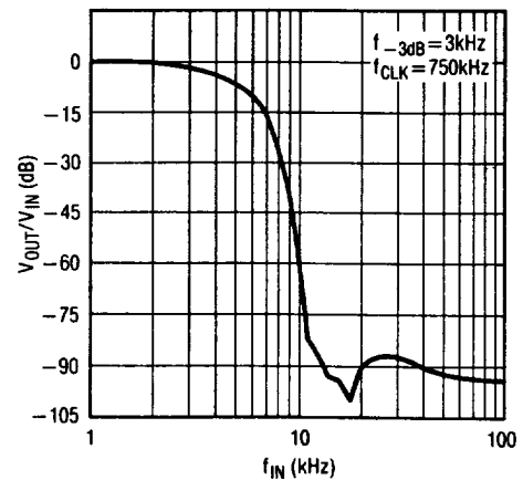
Amplitude Response
