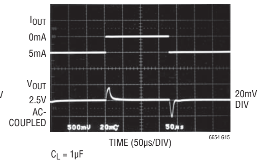
Load Transient Response (Sourcing)
