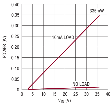
Figure 11. Typical Power Dissipation of the LT6654
