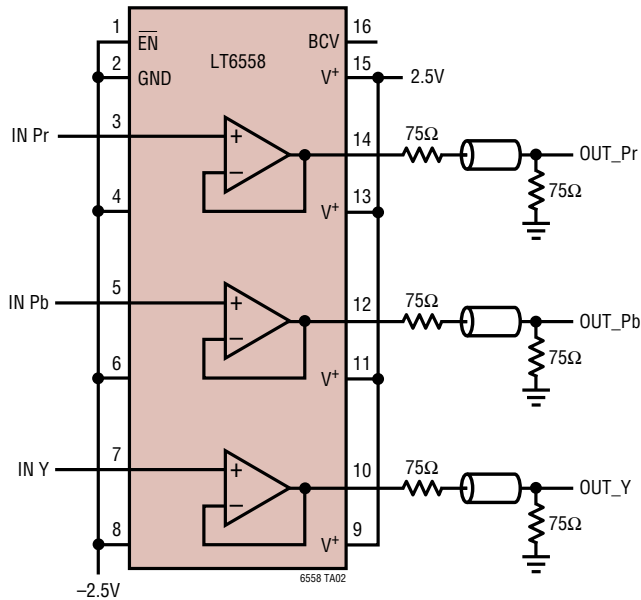
DC-Coupled Split Supply Operation
