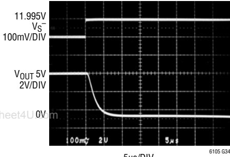
Step Response V_{SENSE} = 100\text{mV to } 5\text{mV}
