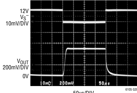
Step Response V_{SENSE} = 0\text{V to } 10\text{mV}, V_S^+ = 12\text{V}
