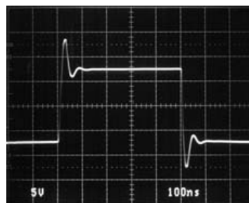
V_S = \pm 15V 100ns/DIV 1995 G34 R_L = 1k
