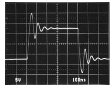
V_S = \pm 15V 100ns/DIV 1995 G35 R_L = 1k
