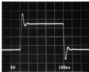
V_S = \pm 15V 100ns/DIV 1995 G33 R_L = 1k
