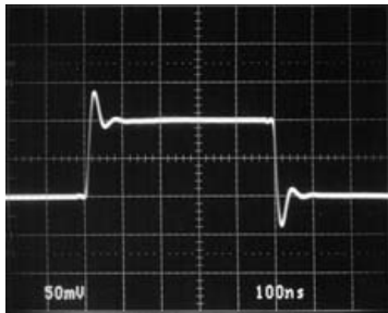
V_S = \pm 15V 100ns/DIV 1995 G30 R_L = 1k
