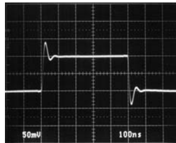
V_S = \pm 15V 100ns/DIV 1995 G31 R_L = 1k
