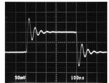
V_S = \pm 15V 100ns/DIV 1995 G32 R_L = 1k
