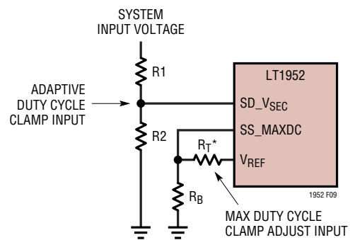
Figure 9. Programming Maximum Duty Cycle Clamp
