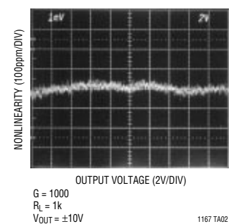
Gain Nonlinearity
