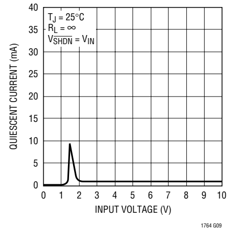
LT1764 Quiescent Current
