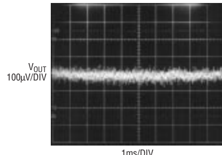
LT1761-5 10Hz to 100kHz Output Noise C_{BYP} = 0.01\mu\text{F}
