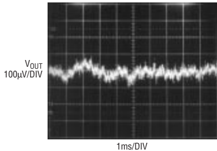
LT1761-5 10Hz to 100kHz Output Noise C_{BYP} = 1000\text{pF}
