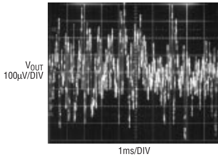
LT1761-5 10Hz to 100kHz Output Noise C_{BYP} = 0
