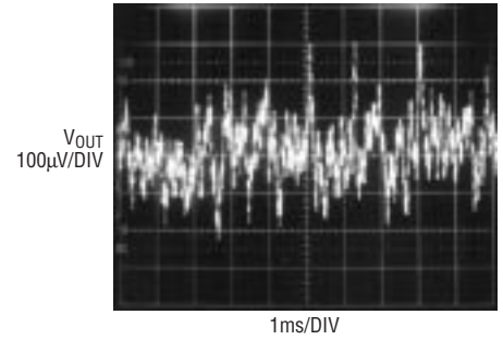
LT1761-5 10Hz to 100kHz Output Noise C_{BYP} = 100\text{pF}
