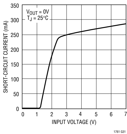
Current Limit
