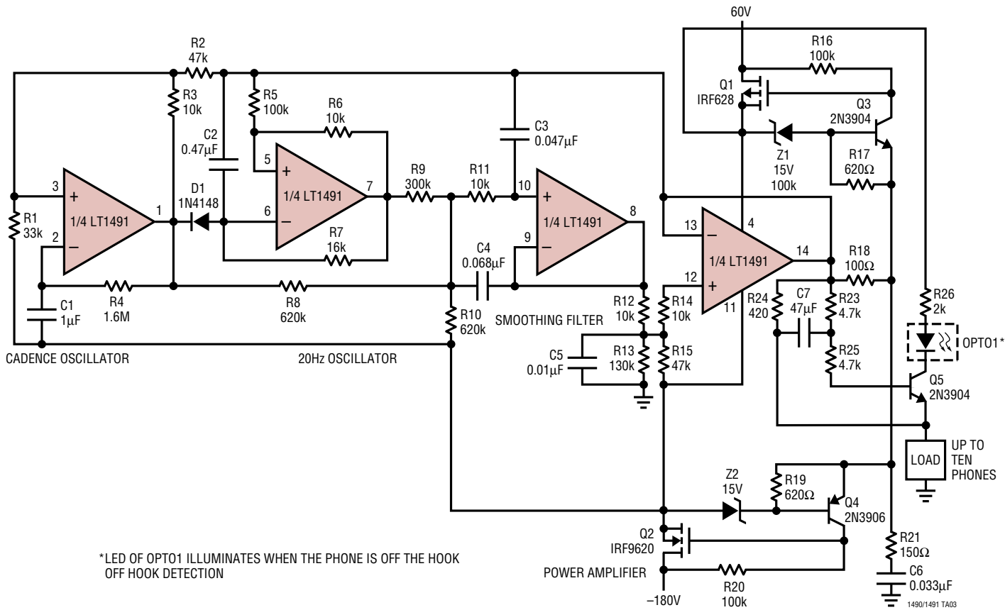
Ring-Tone Generator
