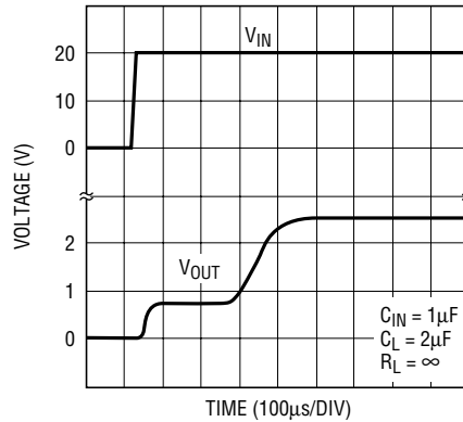
Turn-On Time
