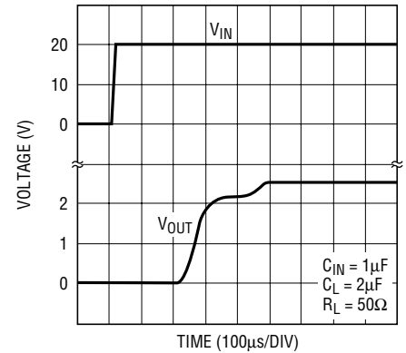
Turn-On Time
