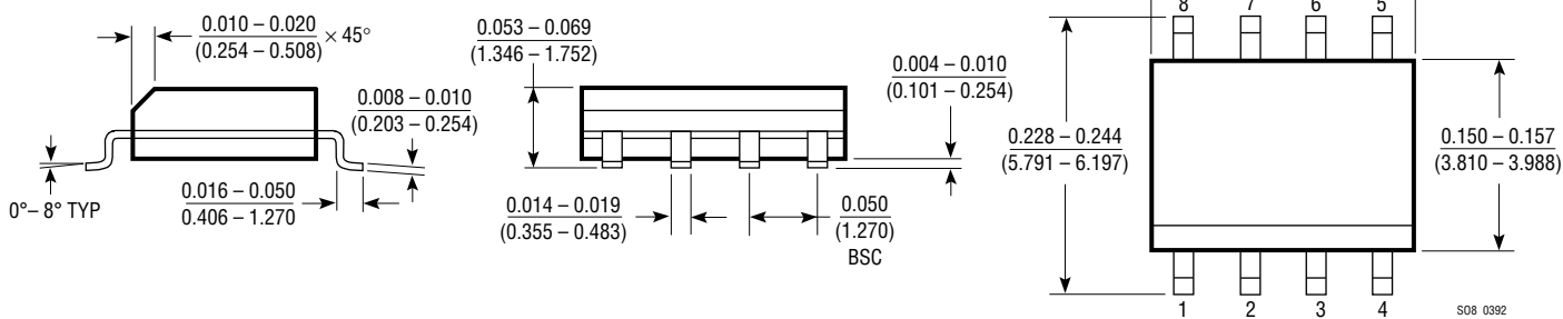
S8 Package, 8-Lead Plastic SOIC
