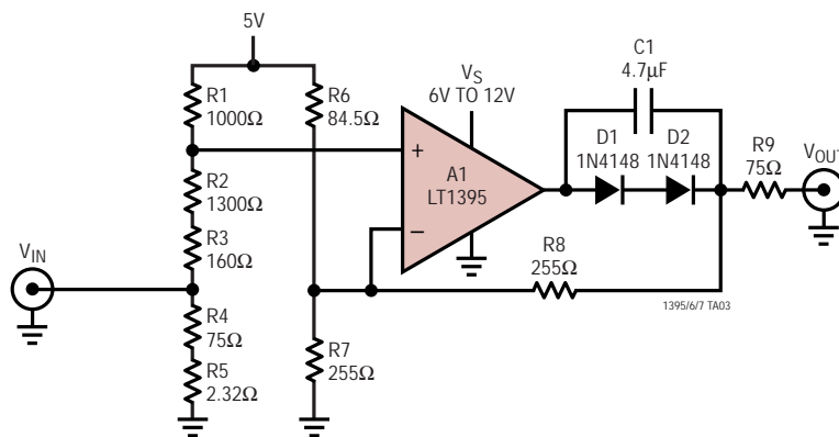
Figure 3. Single Supply RGB Video Amplifier (1 of 4 Channels)
