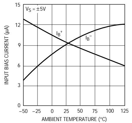
Input Bias Currents vs Temperature
