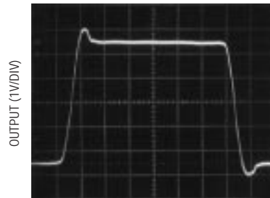
Large-Signal Transient Response ( A_V = -1 )
