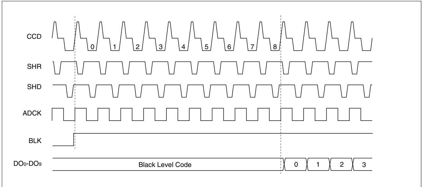
Pixel Data Readout Sequence (1) : Conversion Start
