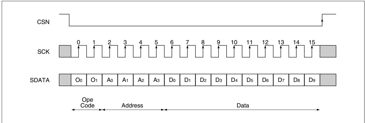
Serial Write Control
