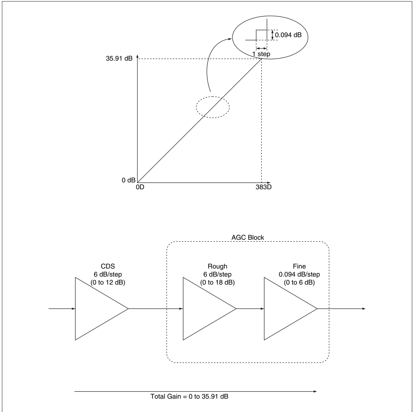
Gain Control
