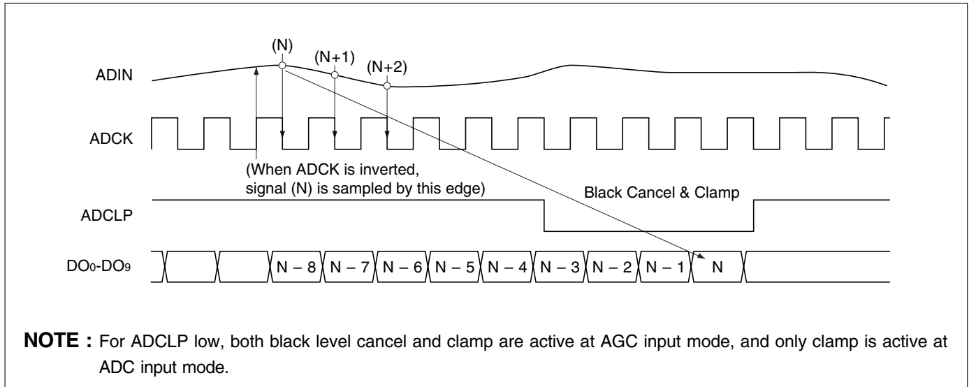
ADIN Signal Processing (AGC Input)
