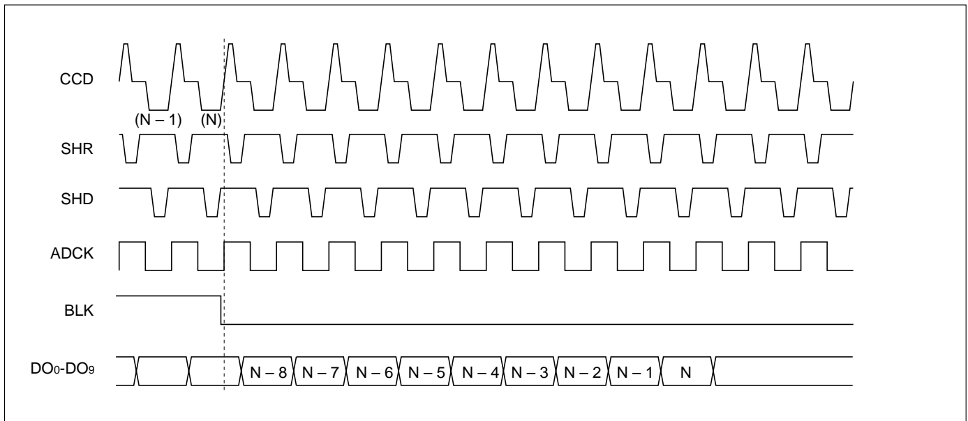
Pixel Data Readout Sequence (2) : Conversion End
