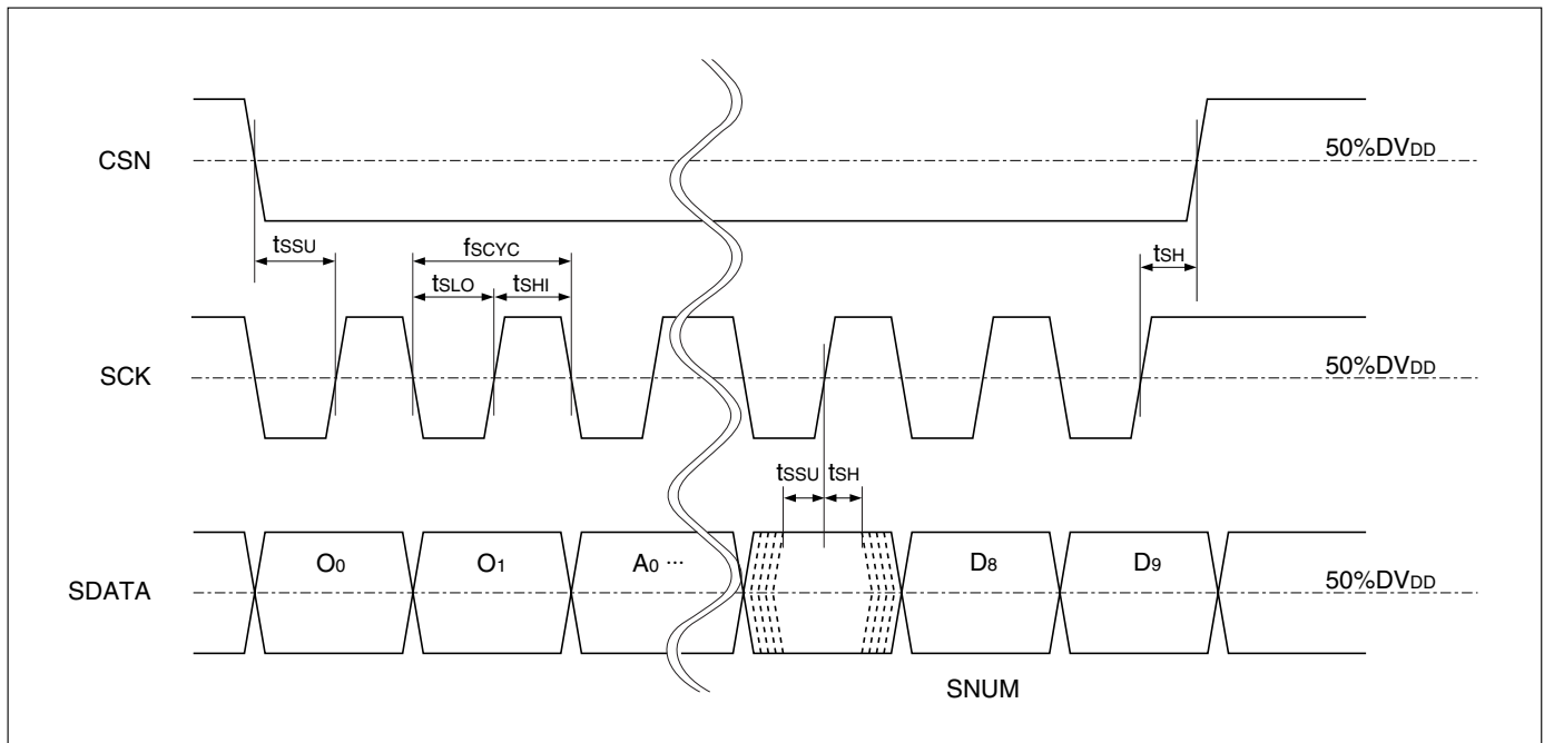
Serial I/F Timing
