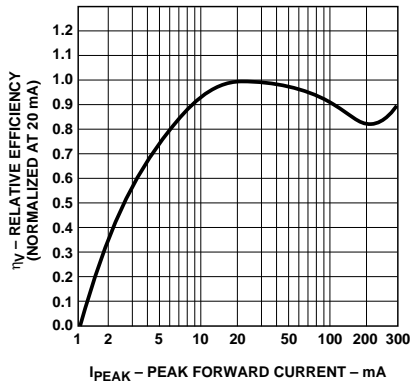
Figure 4. Relative Efficiency vs. Peak Forward Current.
