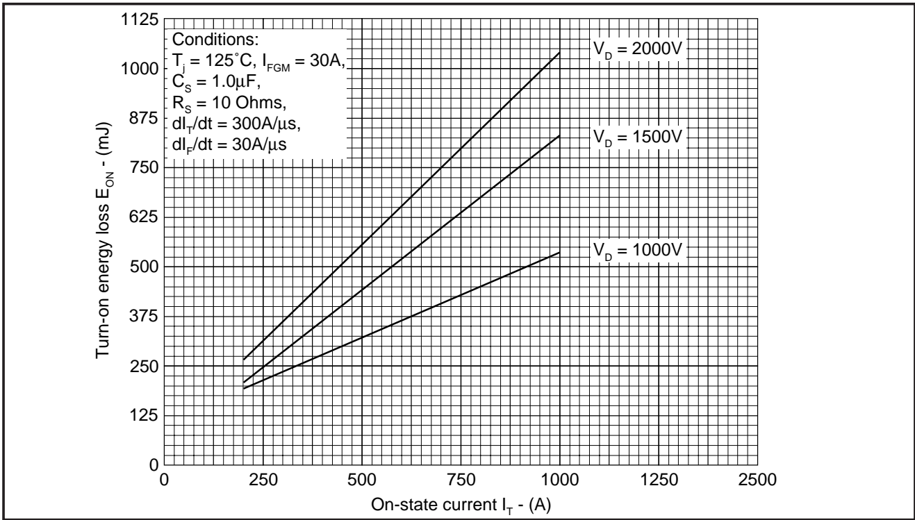
Fig.10 Turn-on energy vs on-state current
