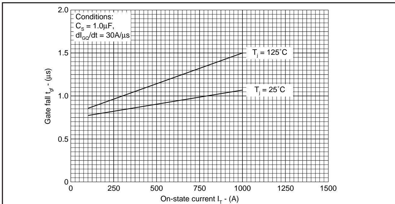
Fig.20 Gate fall time vs on-state current
