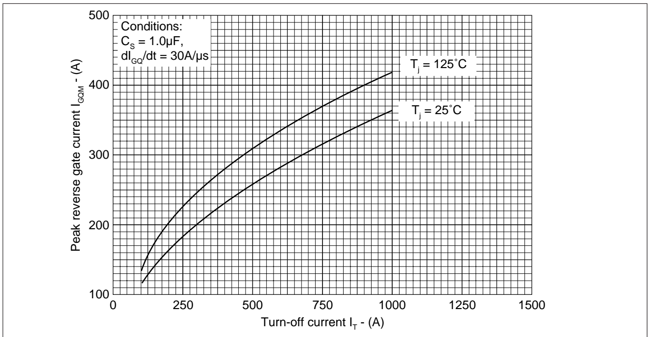
Fig.24 Peak reverse gate current vs turn-off current
