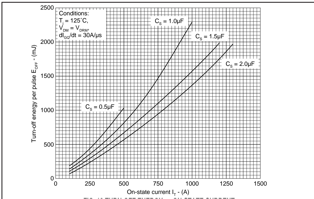
Fig.19 Turn-off energy vs on-state current
