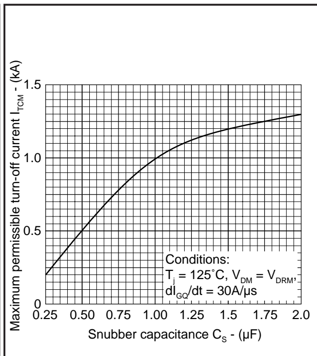
Fig.3 Maximum dependence of I_{TCM} on C_S
