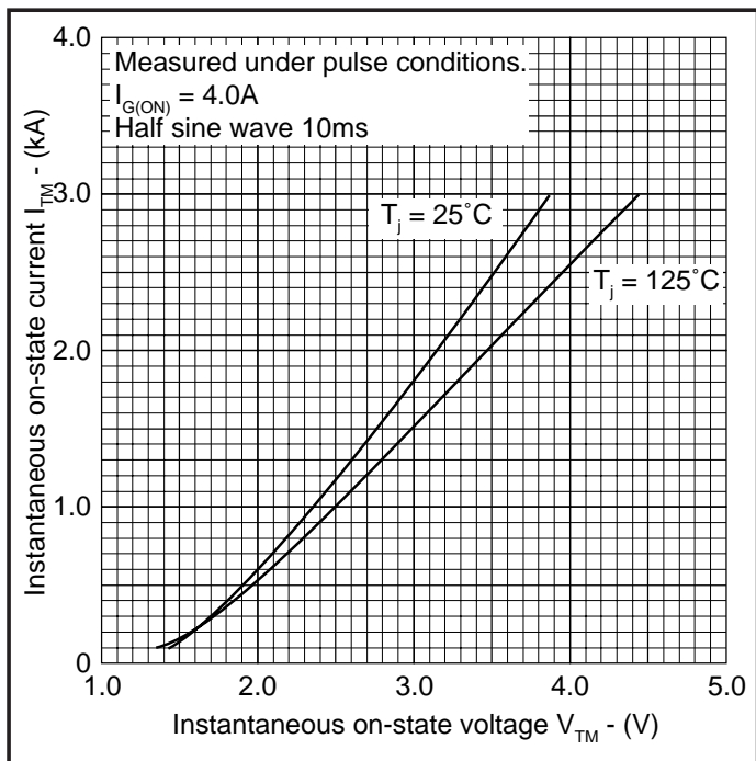
Fig.2 On-state characteristics
