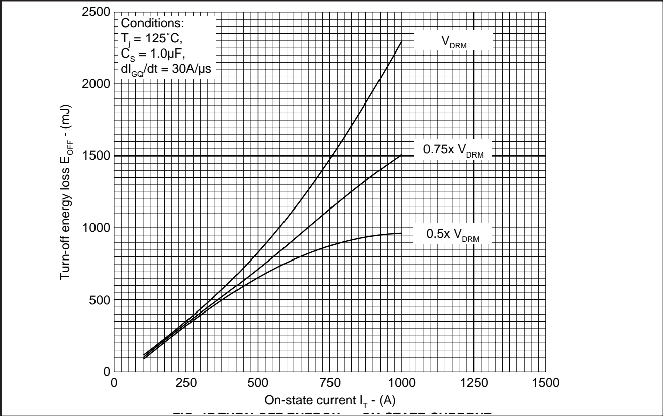
Fig.17 Turn-off energy vs on-state current
