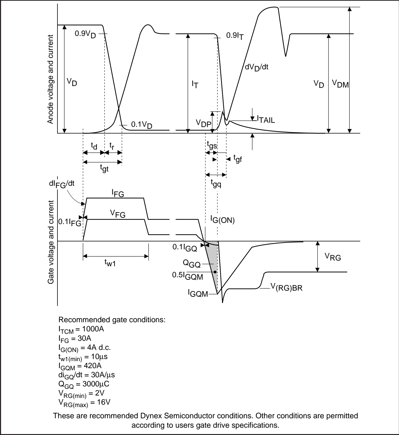
Fig.29 General switching waveforms
