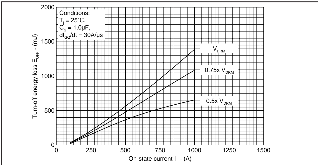
Fig.15 Turn-off energy vs on-state current
