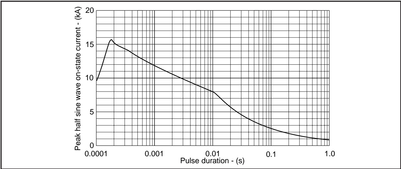
Fig.5 Surge (non-repetitive) on-state current vs time
