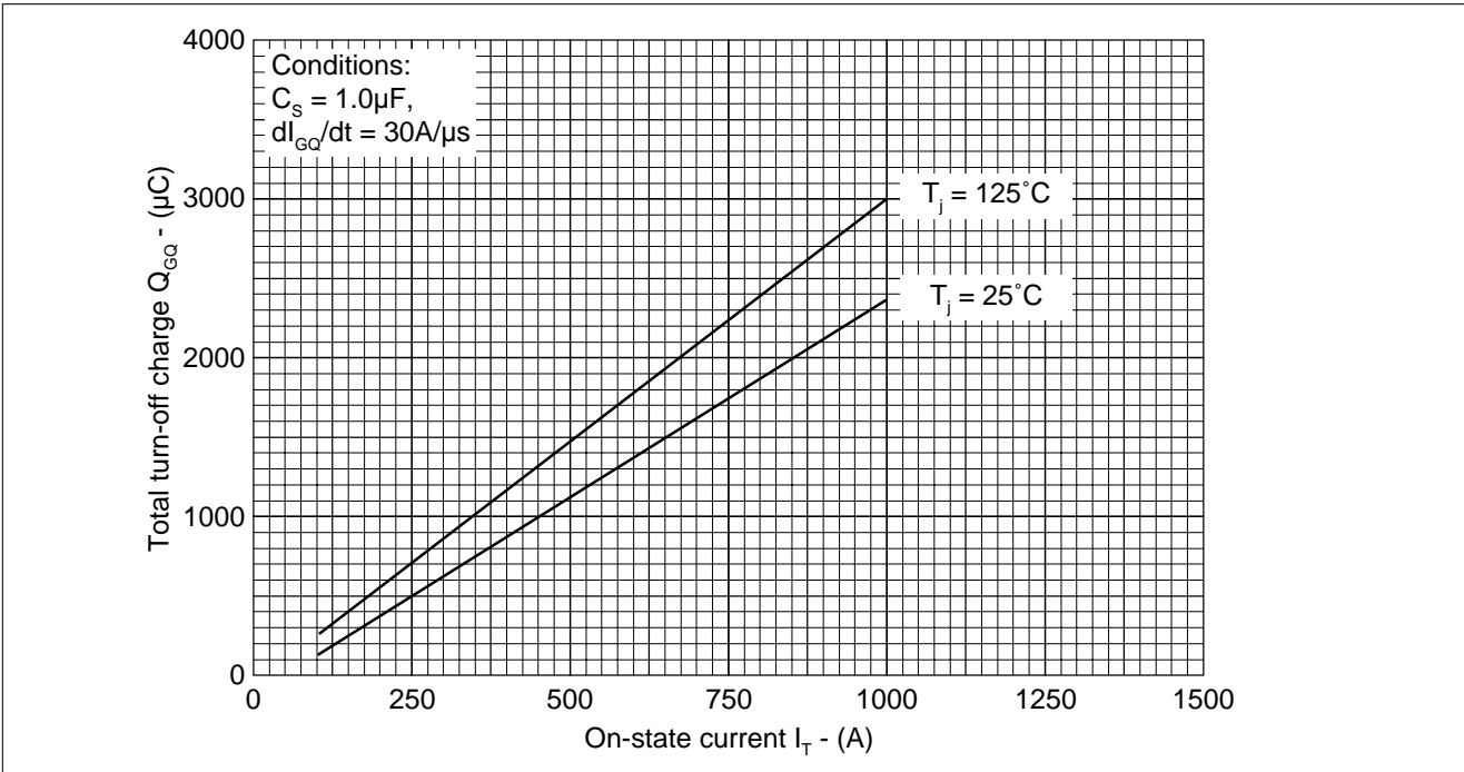
Fig.26 Turn-off gate charge vs on-state current
