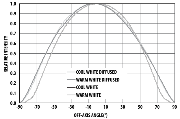
Figure 4. Radiation Pattern
