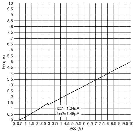
Current consumption
