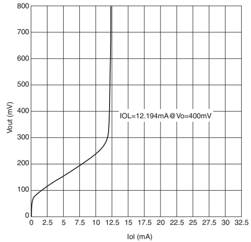
'L' output current
