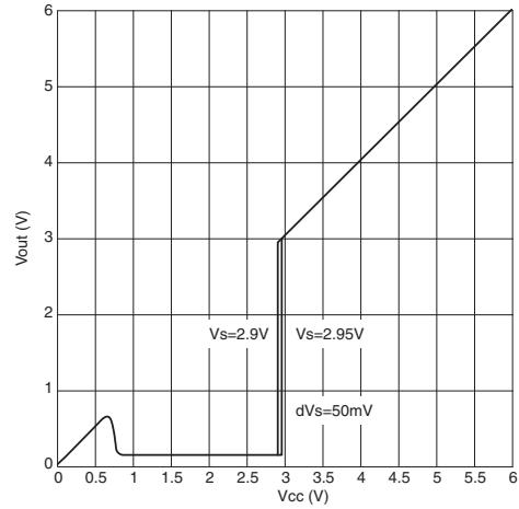
I/O characteristic
