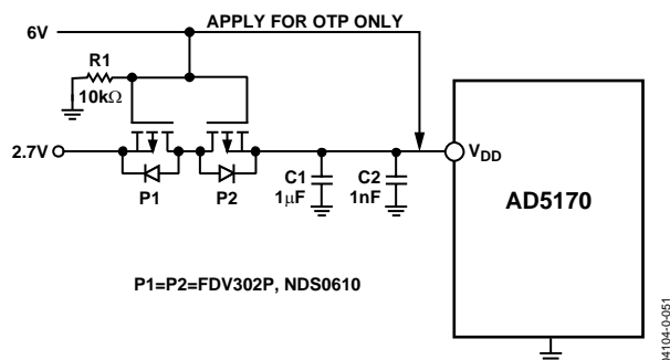
Figure 39. Isolate 6 V OTP Supply from 2.7 V Normal Operating Supply. The 6 V supply must be removed once OTP is completed
