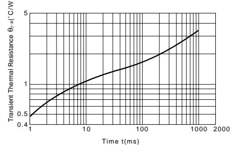
θj-a-t Characteristics
