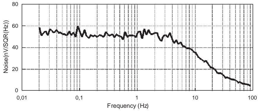
Noise = F(frequency)
