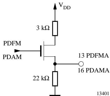
Figure 6. Analog outputs PDFMA, PDAMA
