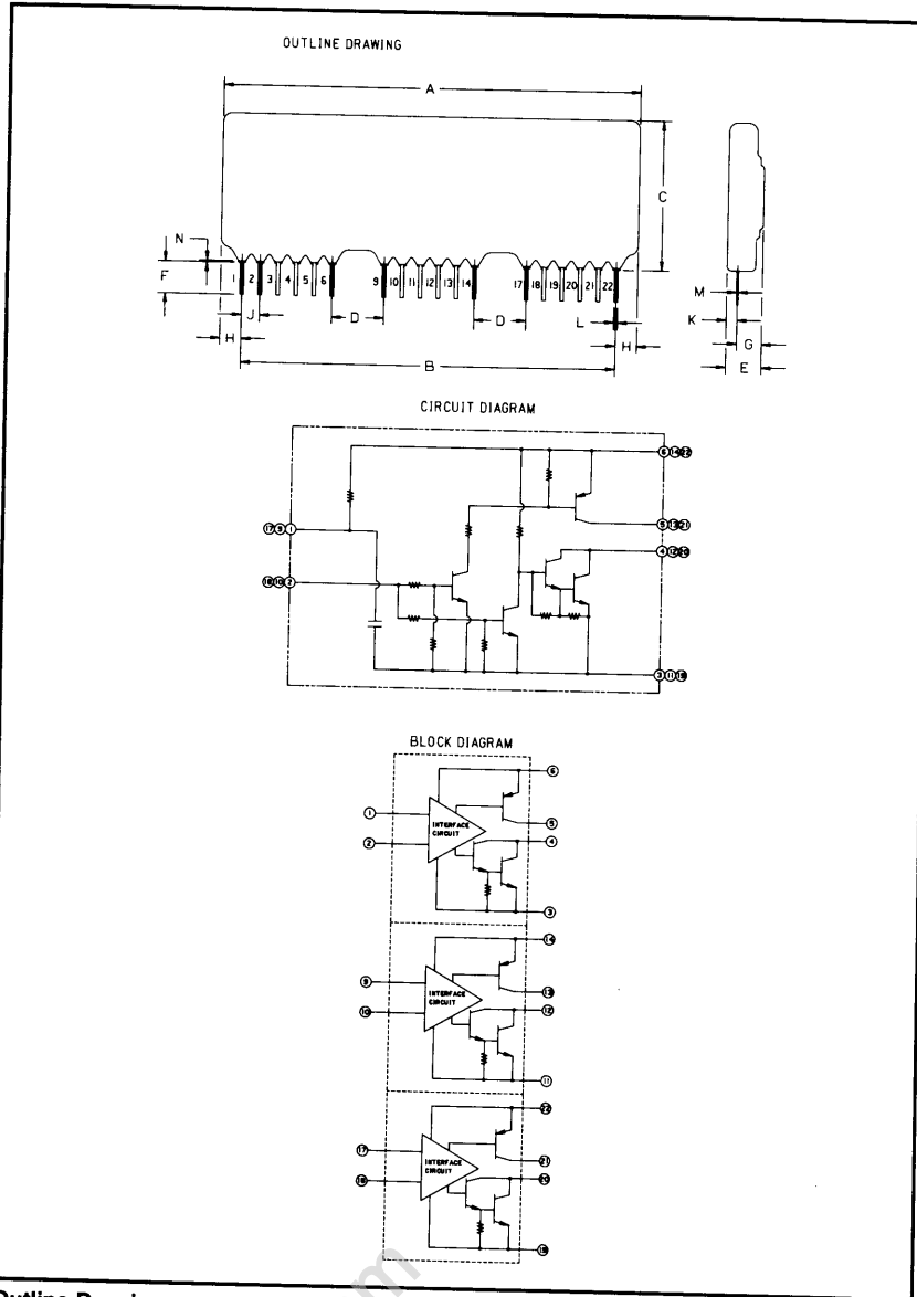
Outline Drawing
