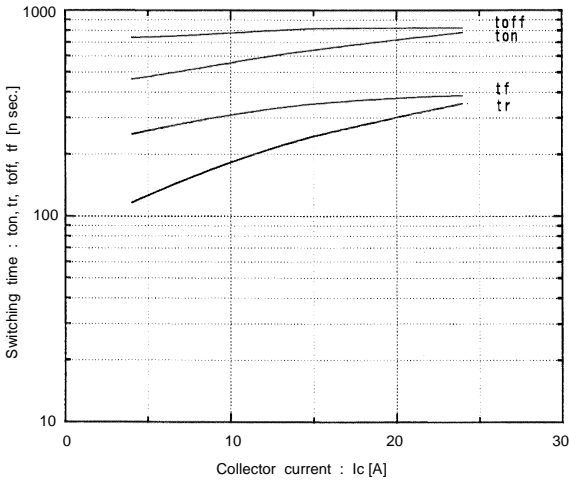
Switching time vs. Collector current V cc =600V, R G =82 ohm, V GE =±15V, T j =25°C
