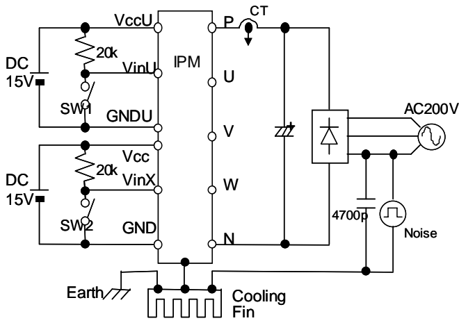
Figure 6. Switching Characteristics Test Circuit
