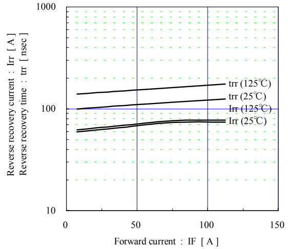
Reverse recovery characteristics (typ.) Vcc=600V, VGE=±15V, Rg=9.1Ω
