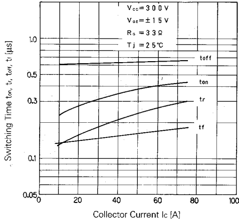
Switching Time
