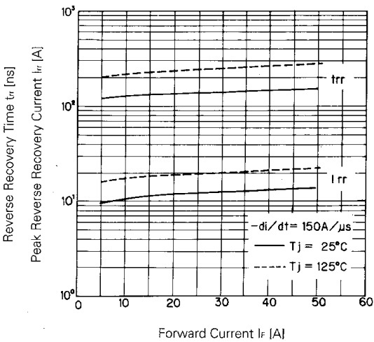
T_{rr}, I_{rr}-I_f
