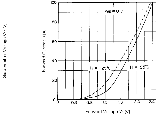
Forward Voltage of Free Wheel Diode
