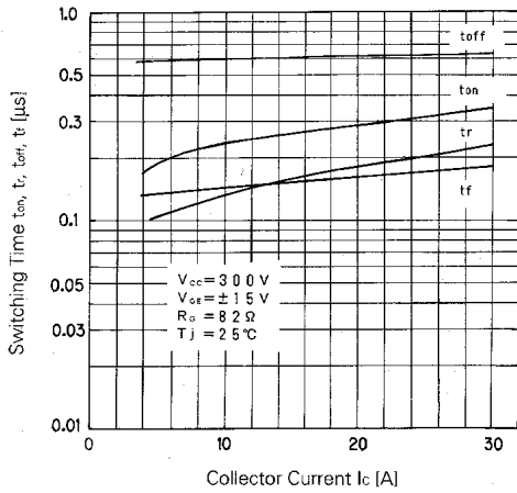
Switching Time
