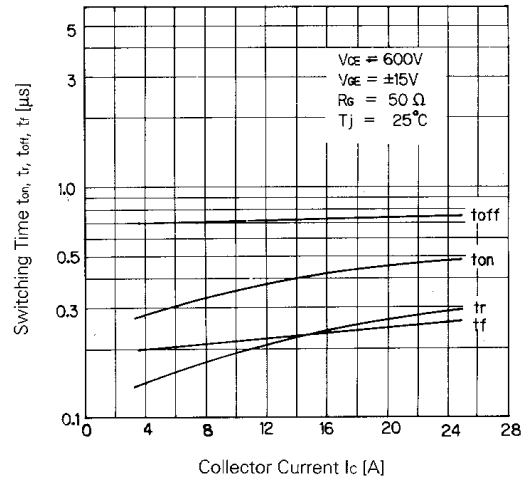
Switching Time
