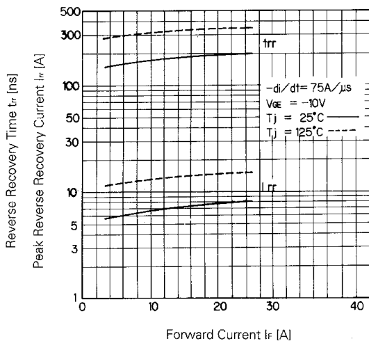
t_{rr}, I_{rr}-I_f
