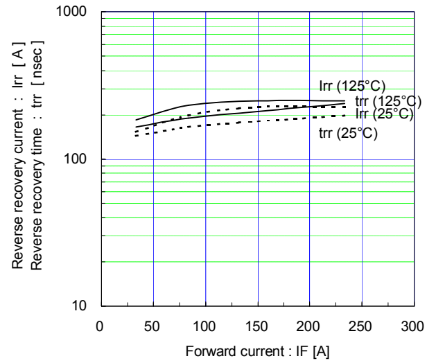
Reverse recovery characteristics (typ.) V_{cc}=900\text{V} , V_{GE}=\pm 15\text{V} , R_g=3.3\Omega
