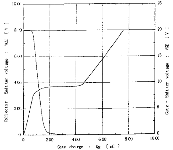
Dynamic Gate charge (typ.) Vce=800V, Ic=100A, Tj= 25°C
