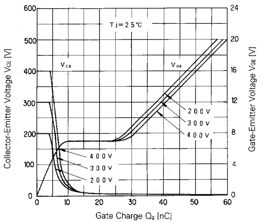
Dynamic Input Characteristic
