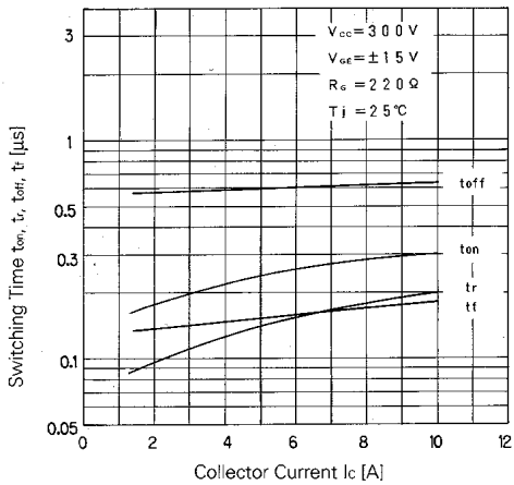
Switching Time
