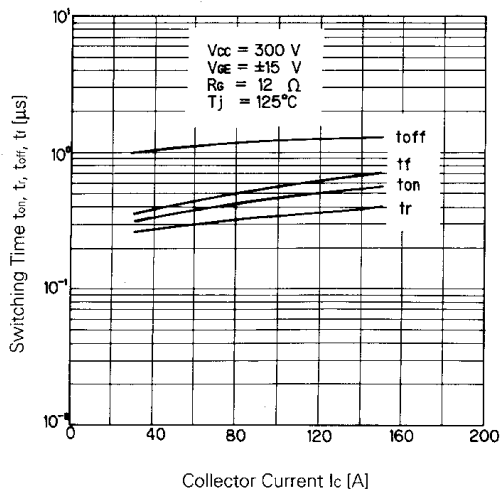
Switching Time
