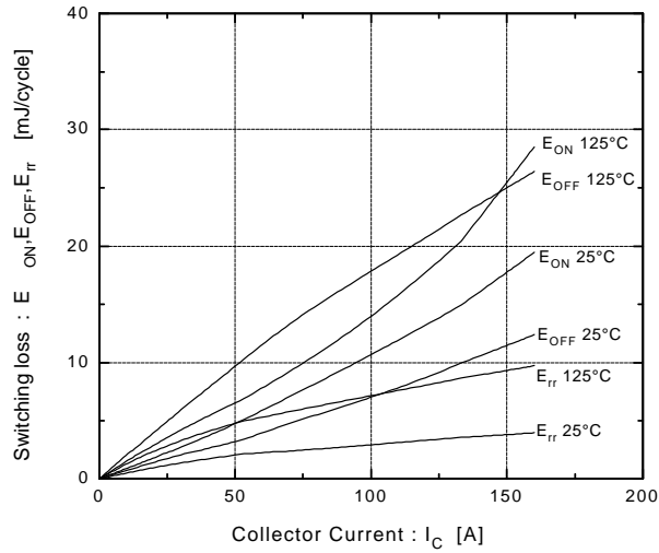
Switching loss vs. Collector current V_{CC}=600V, R_G=9.1\Omega, V_{GE}=\pm 15V
