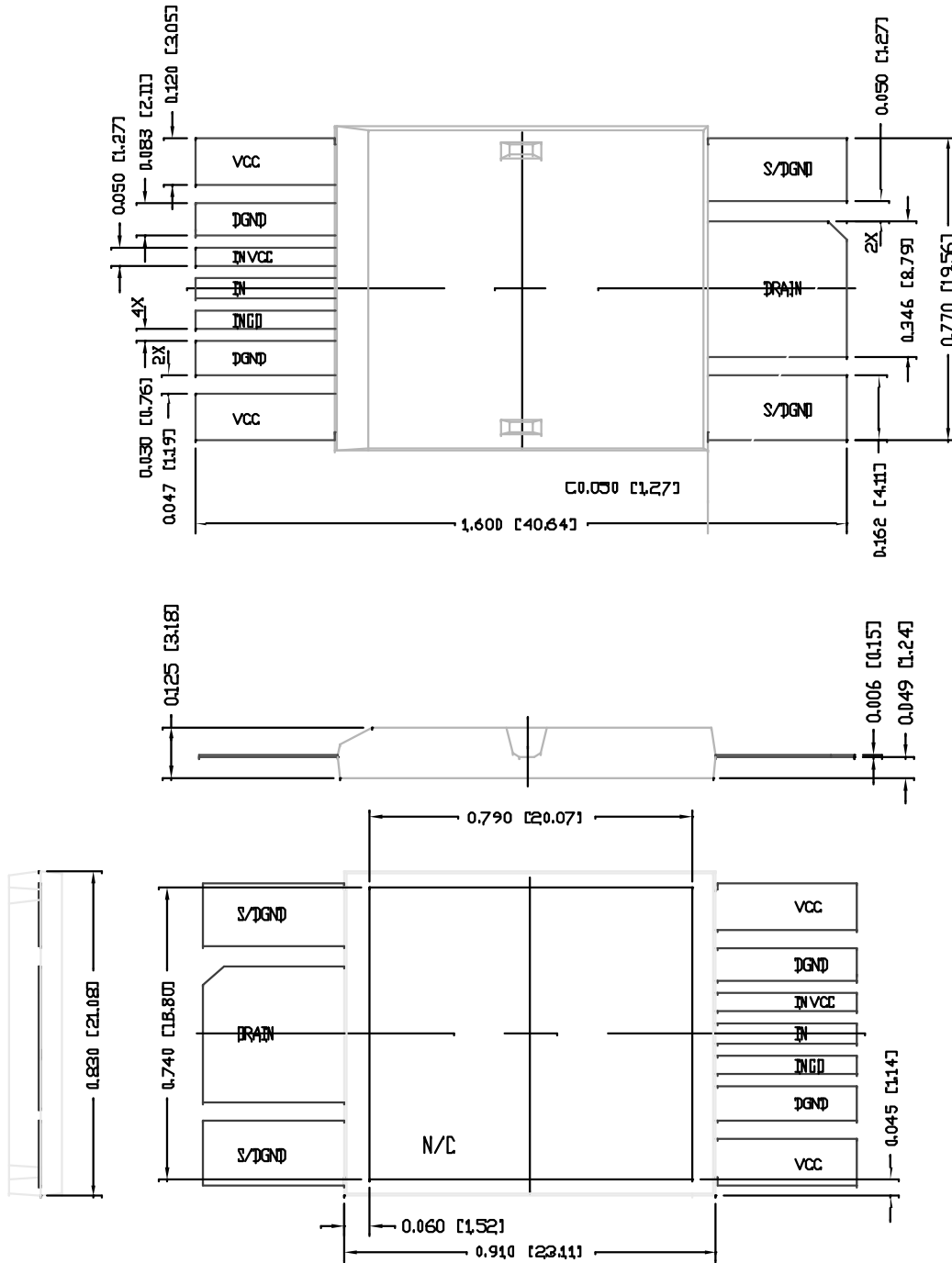
Fig. 16 IXZ4DF18N50 Package Outline
