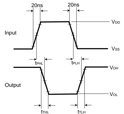
Fig. 2 Switching characteristics
