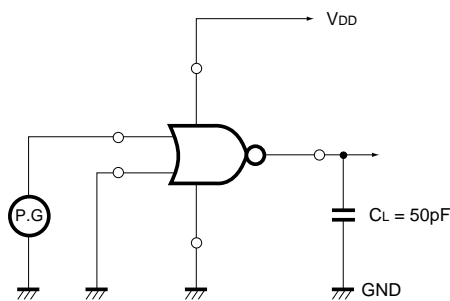
Fig.2 Switching characteristics
