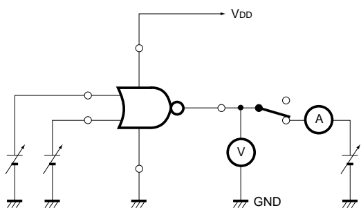
Fig.1 DC characteristics
