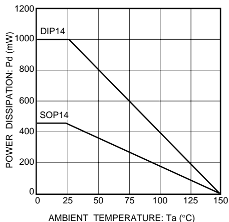
Fig.3 Power dissipation vs. Ta characteristic
