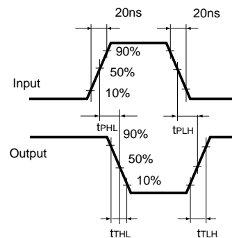
Fig.2 Switching characteristics
