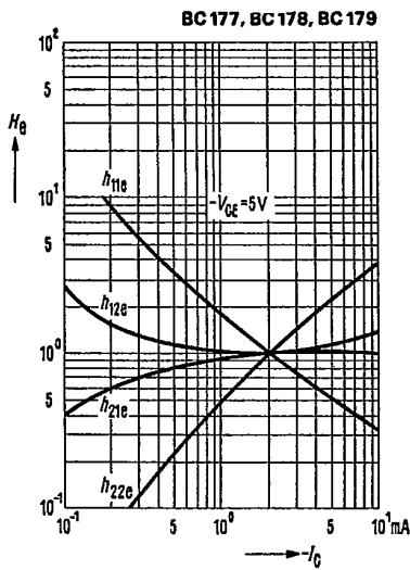
h -parameter vs. collector current -V_{CE} = 5V; T_{amb} = 25^\circ C
