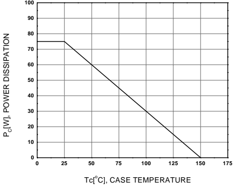
Figure 7. Power Derating
