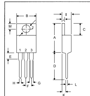
TO-220AB
