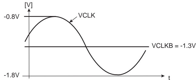
Figure 31. Single-ended Clock Input (ECL): VCLK Common Mode = -1.3\text{V} ; VCLKB = -1.3\text{V}
