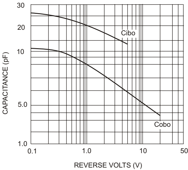
Fig. 3 Typical Capacitance
