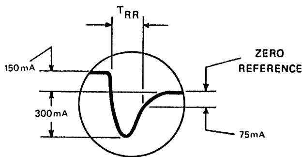
TYPICAL REVERSE RECOVERY WAVEFORM
