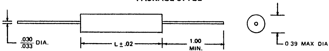
FIG. 3 PACKAGE STYLE
