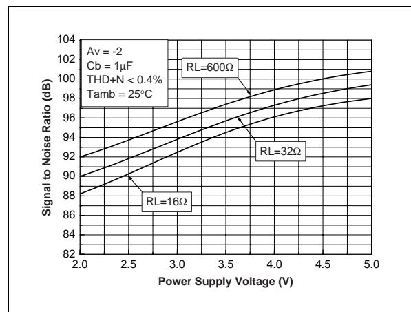
Fig. 74: Signal to Noise Ratio vs Power Supply Voltage with Weighted Filter Type A
