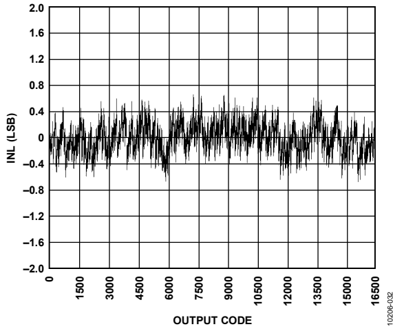
Figure 33. INL, f_{IN} = 9.7 \text{ MHz} , f_{SAMPLE} = 40 \text{ MSPS}
