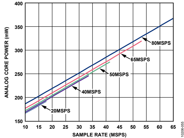
Figure 56. Analog Core Power vs. f_{SAMPLE} for f_{IN} = 9.7 \text{ MHz}
